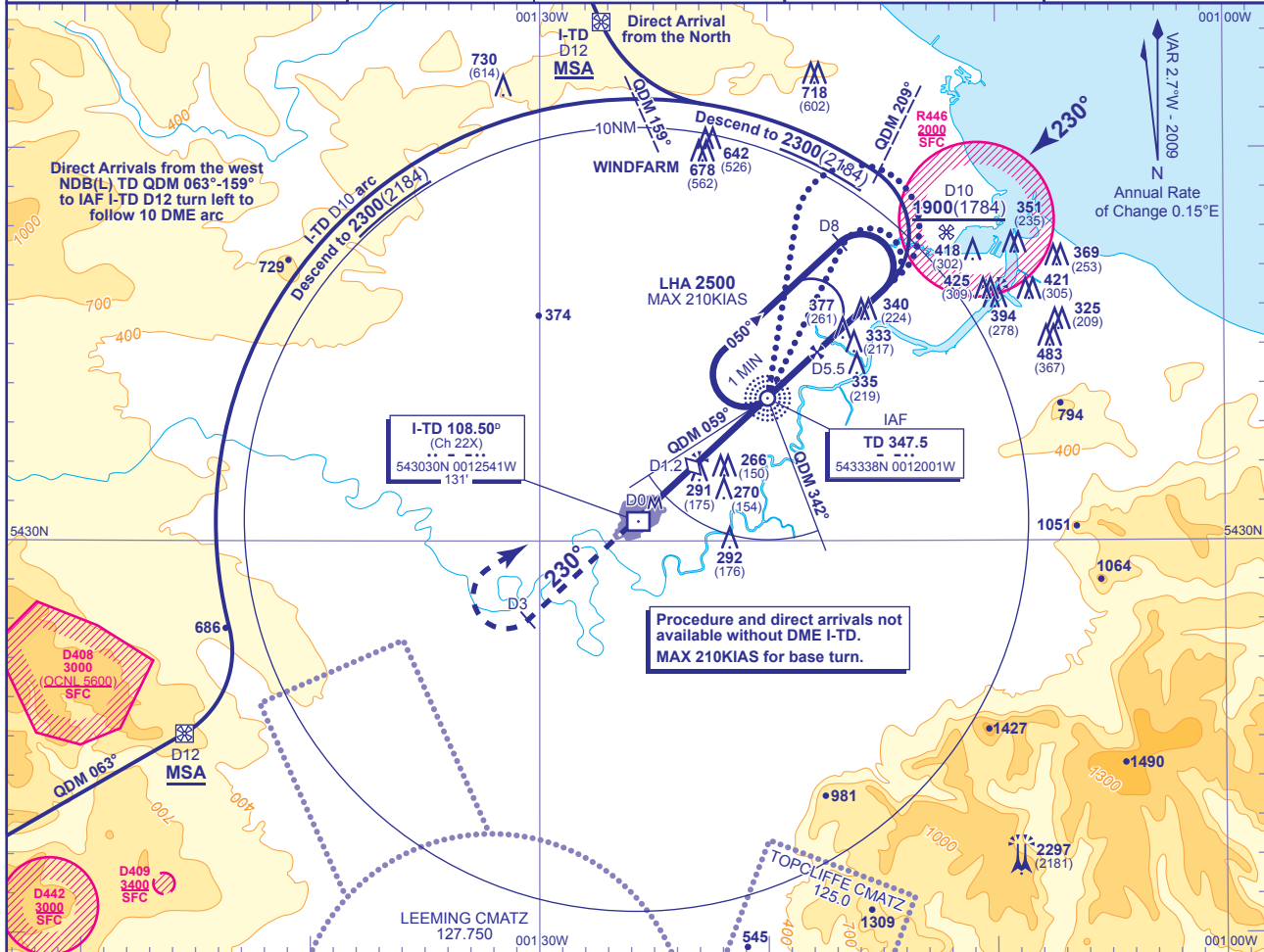
RECOMMENDED PROFILE Gradient 5.19%, 315FT/NM
